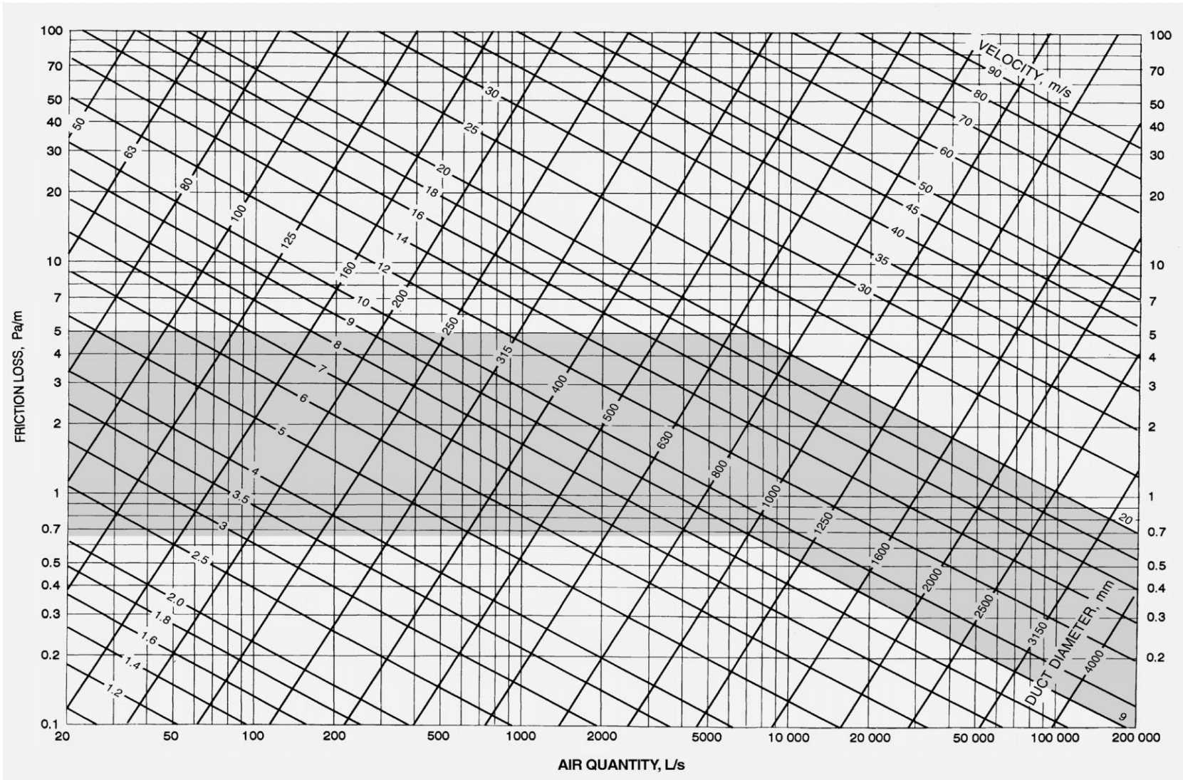
Fig. 9-2 SI Friction of Air in Straight Ducts (Figure 9, Chapter 21, 2013 ASHRAE Handbook—Fundamentals)
